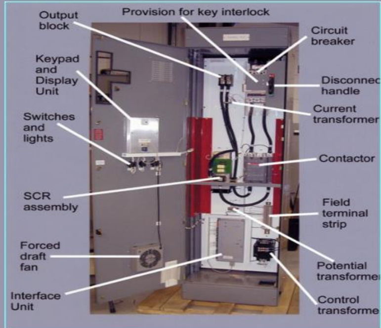
Control Cabinet
